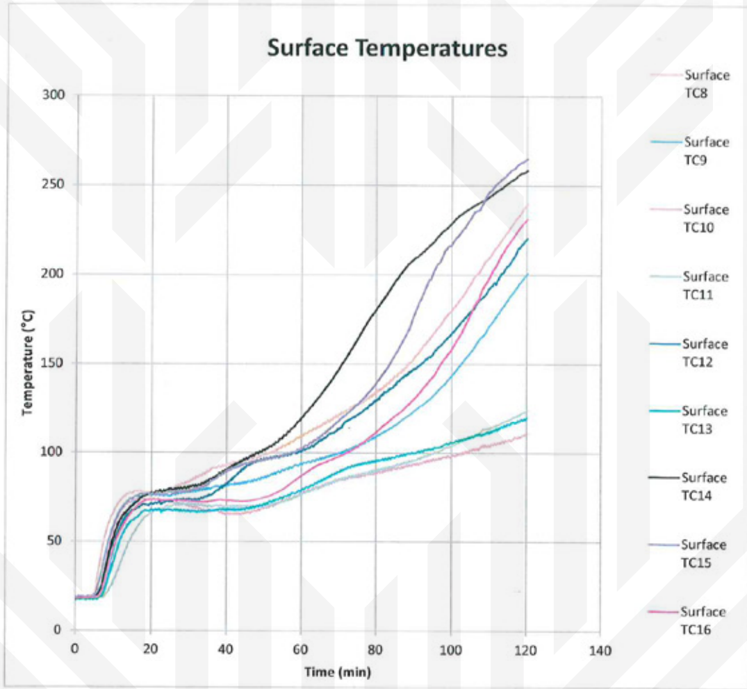
Figure B3: Surface temperatures (Thermocouple sensors for maximum temperature)
