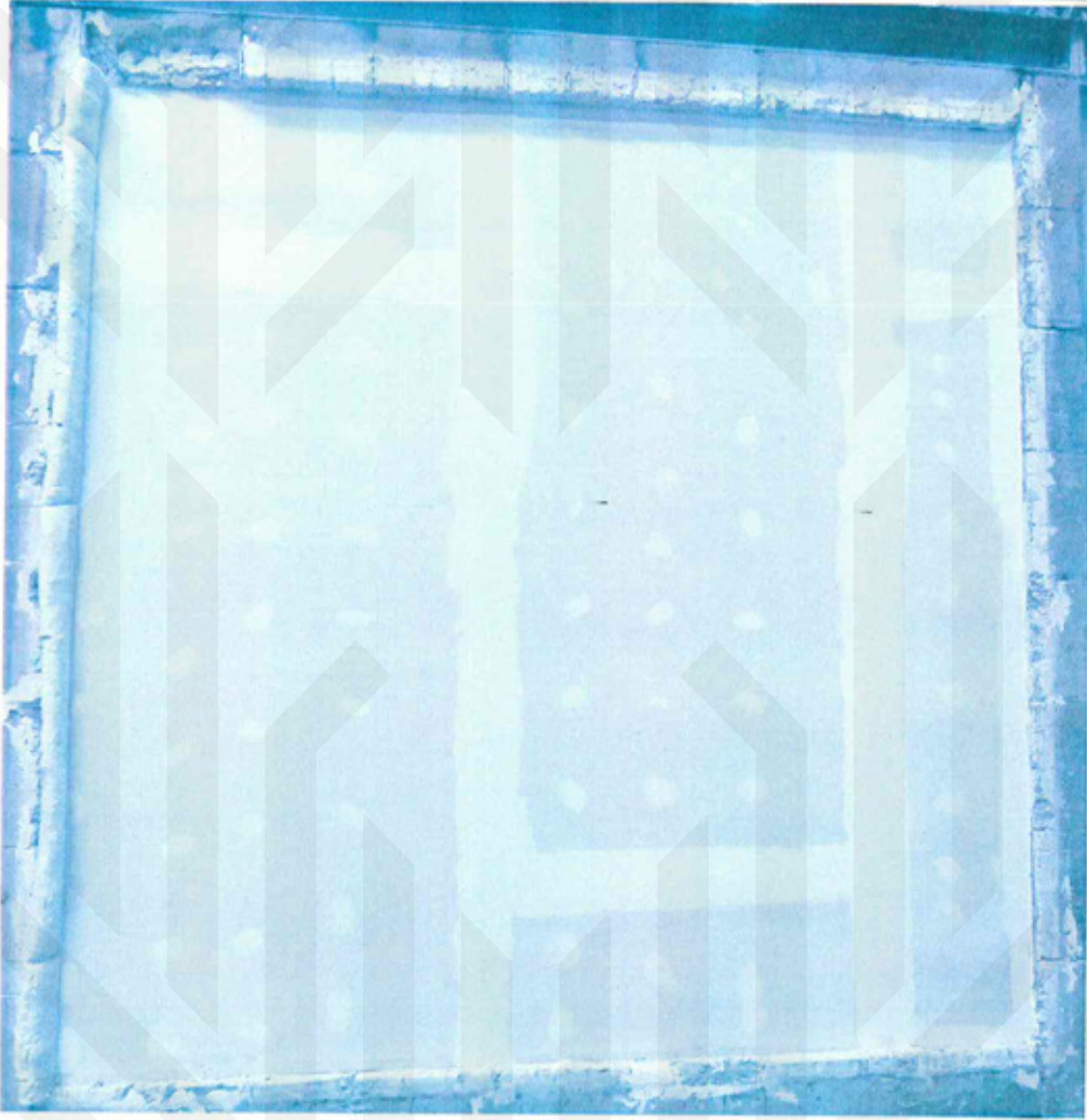
Photo C2: Exposed side of the test specimen before the test
