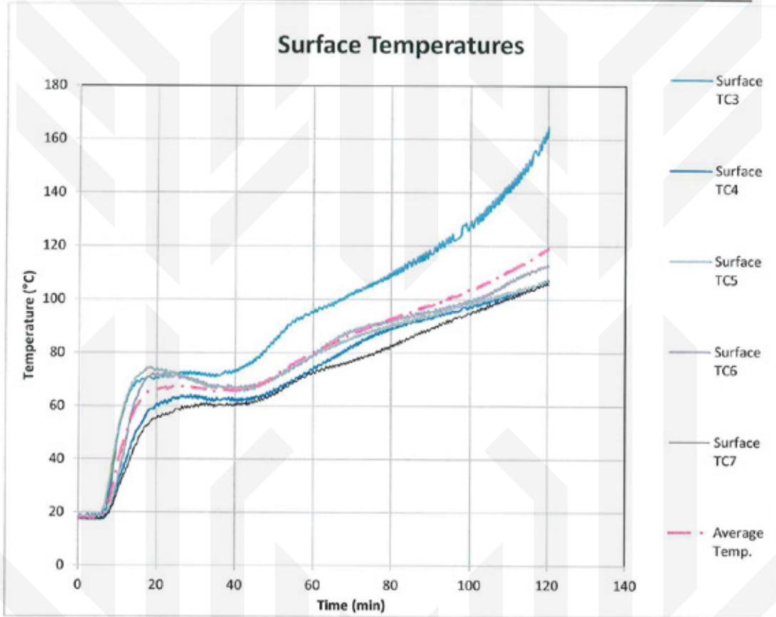
Figure B2: Surface temperatures (Thermocouple sensors for average temperature)
