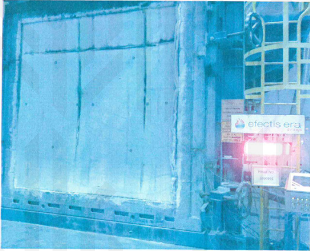
Photo C4: Unexposed side of the test specimen after the test
